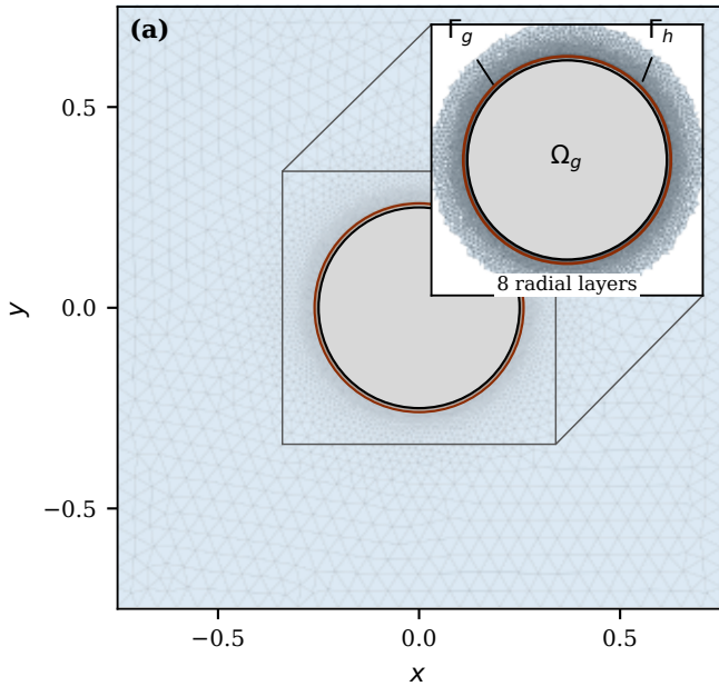
Resolved thin coating
