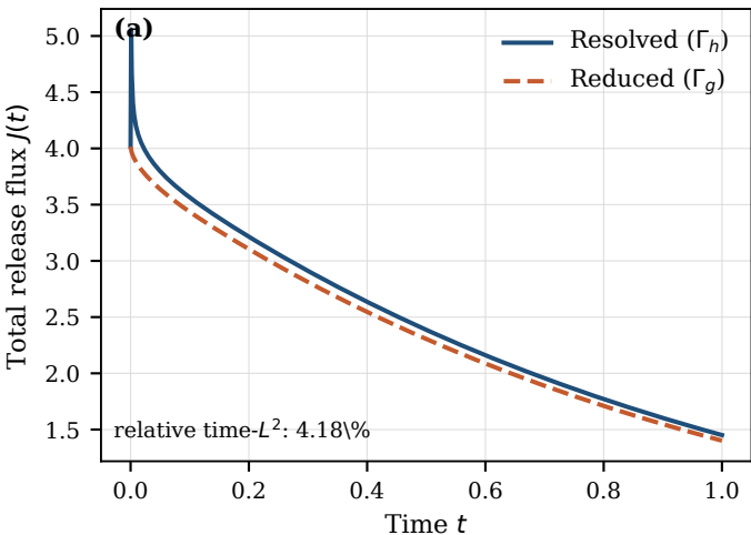
Release flux
