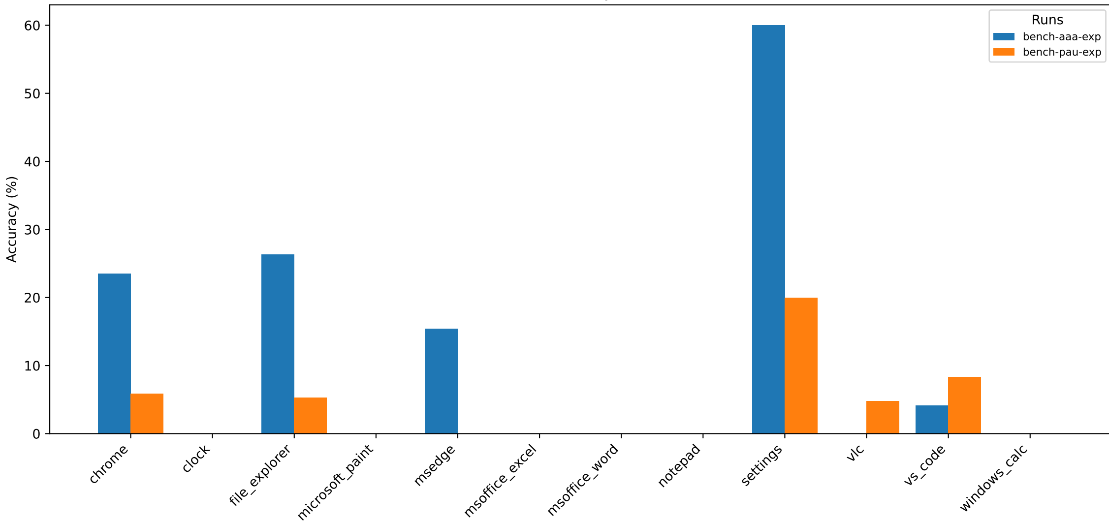
Per-domain Accuracy Across Runs
