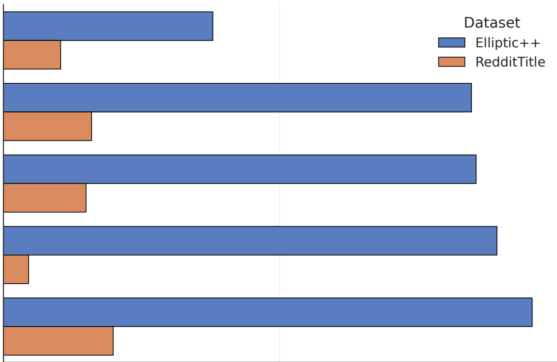
Inference Time
