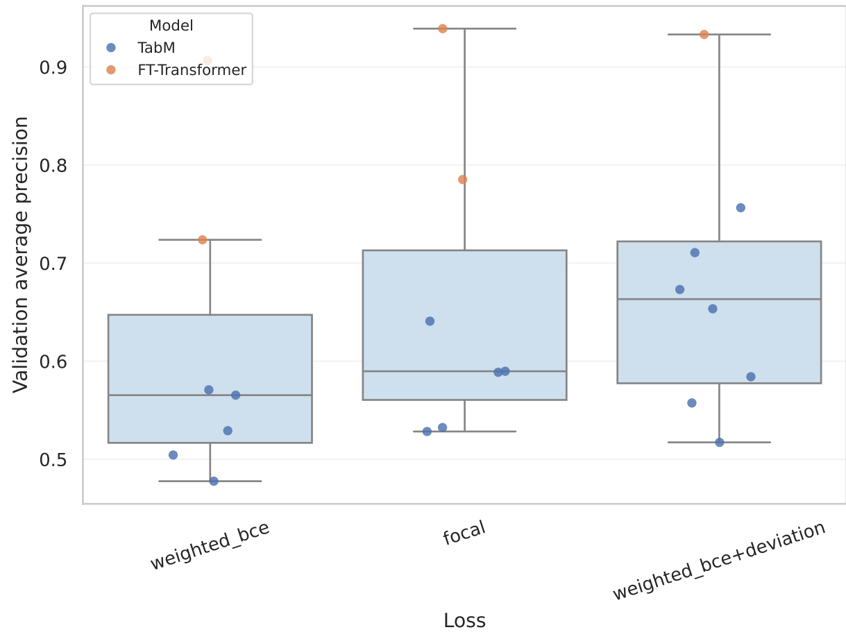
Deep models: loss function
