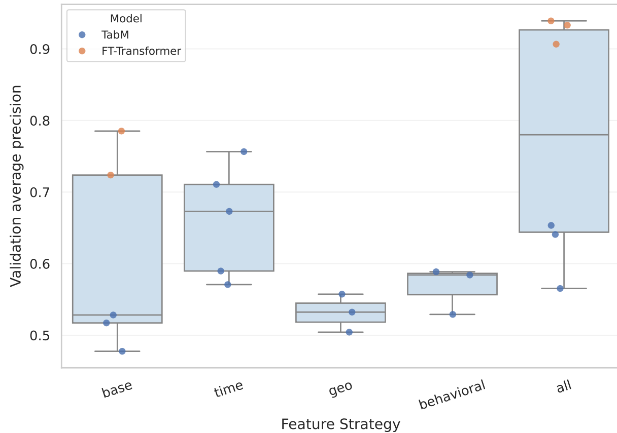
Deep models: feature strategy
