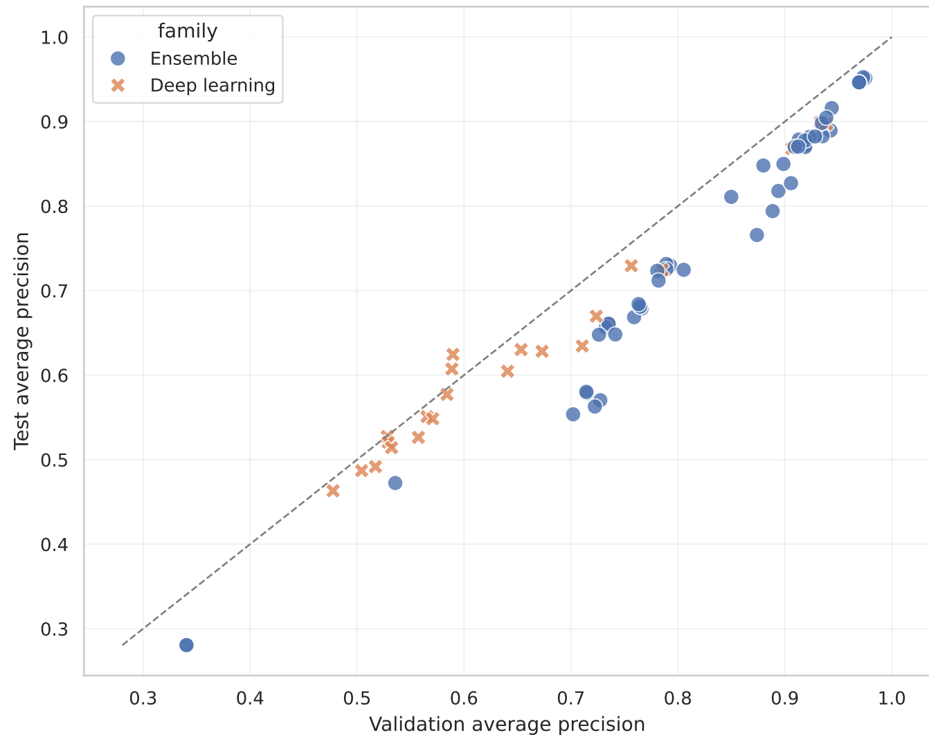
Validation-to-test relationship
