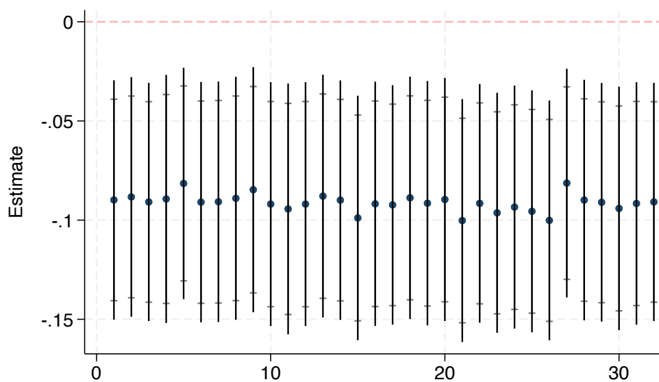
(a) ROA
