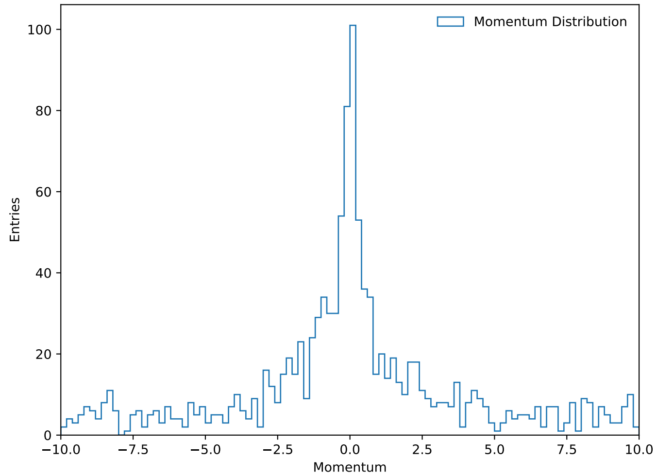
Momentum Distribution
