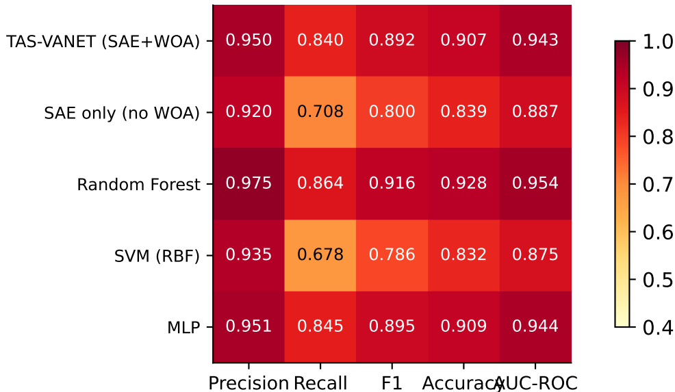
Mean Performance Across All CV Folds
