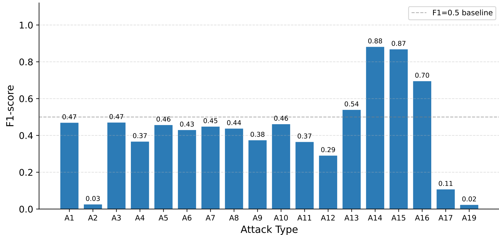
Per-Attack-Type Detection F1 — TAS-VANET (held-out test set)
