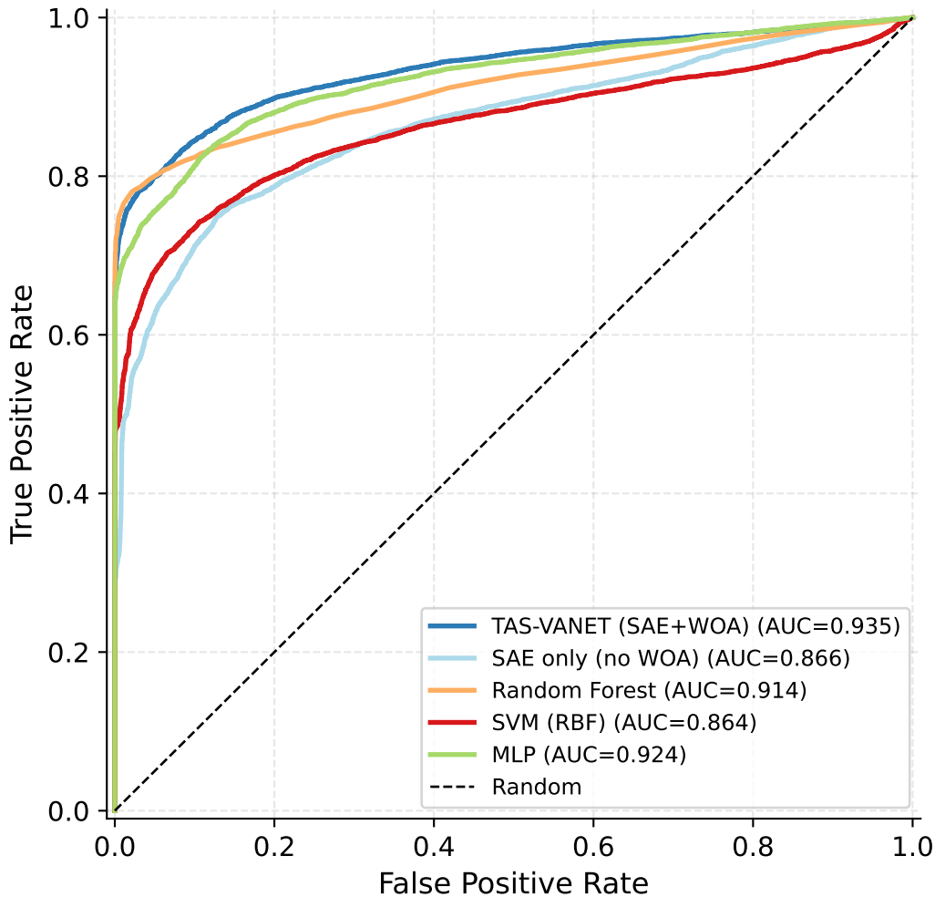
ROC Curves — Held-out Test Set
