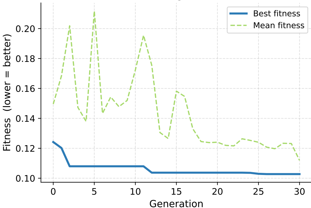
WOA Convergence Curve
