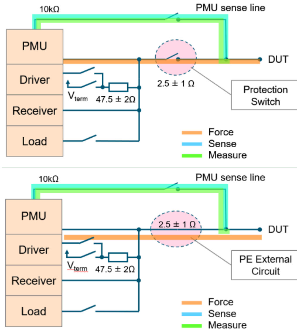
PS5000 receiver: Simplified diagram of the pin electronics
