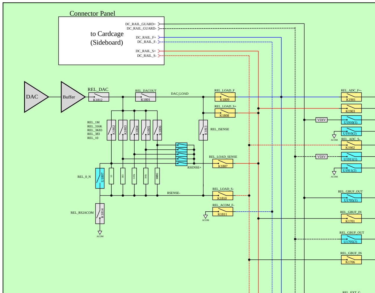
The system control board diagram
