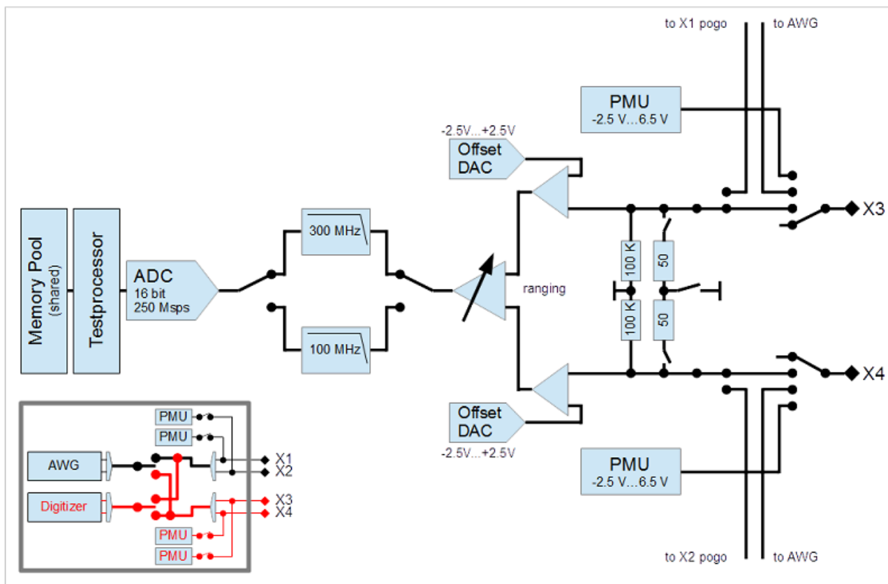
WSMX block diagram of the high-speed digitizer
