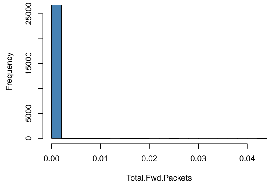
Distribution: Total.Fwd.Packets
