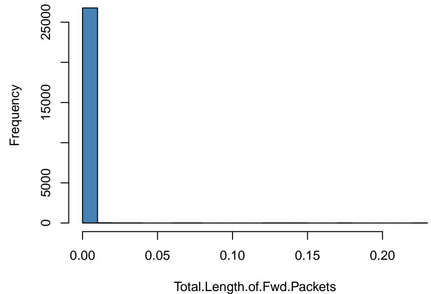
Distribution: Total.Length.of.Fwd.Packets
