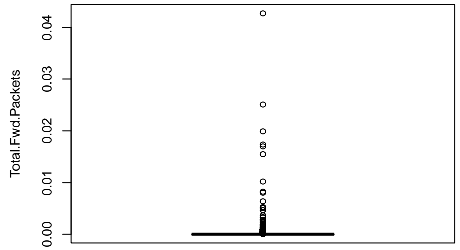
Total.Fwd.Packets
