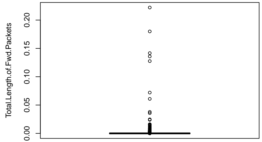
Total.Length.of.Fwd.Packets
