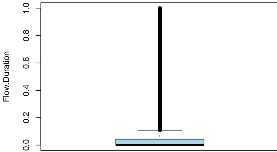
Flow.Duration
