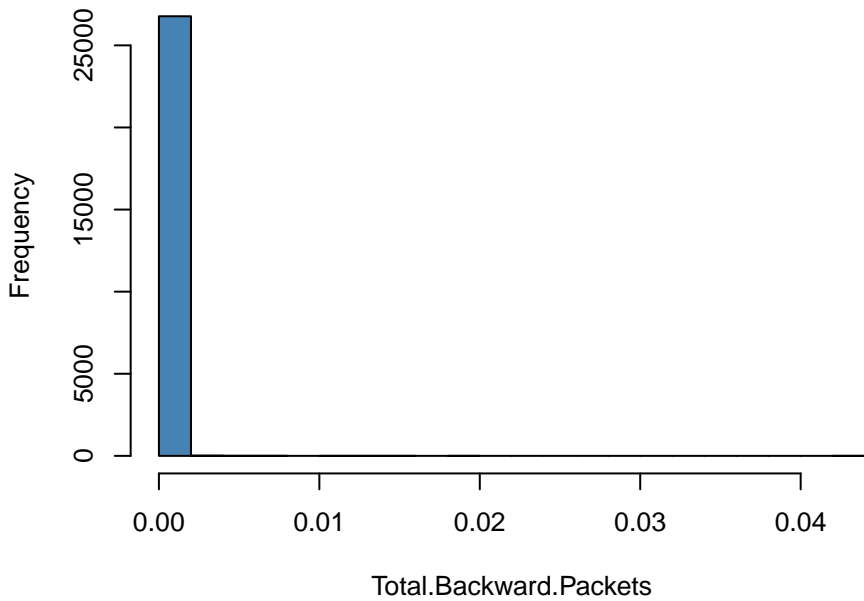
Distribution: Total.Backward.Packets
