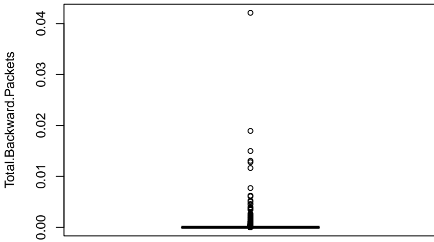
Total.Backward.Packets
