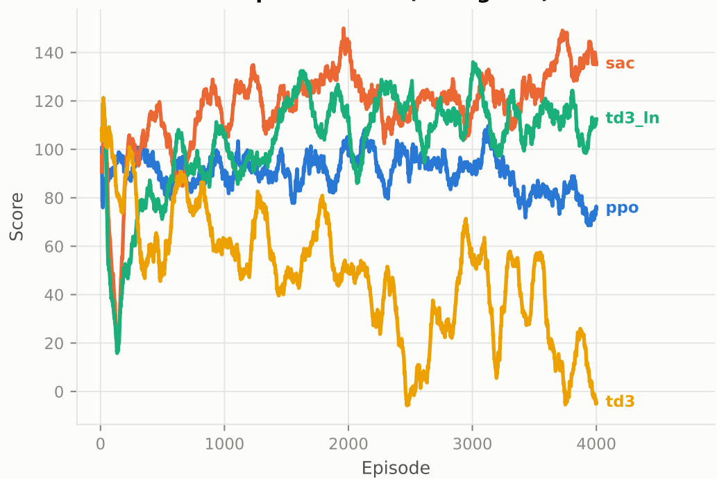
Episode score (rolling 100)
