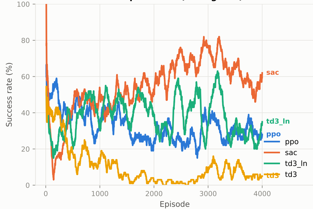
Grasp success (rolling 100)
