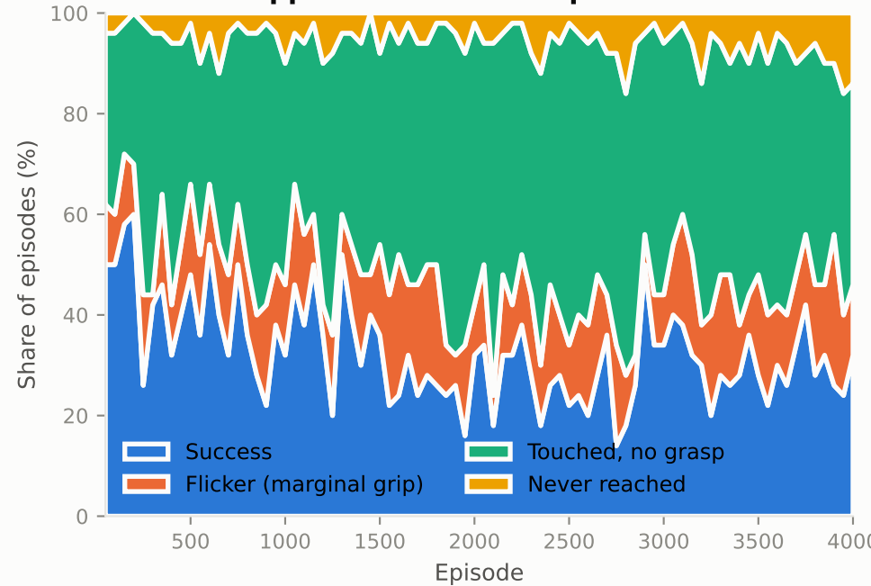
ppo — outcome composition
