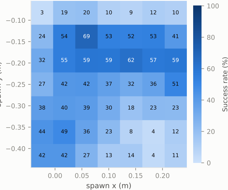
ppo — success by spawn position
