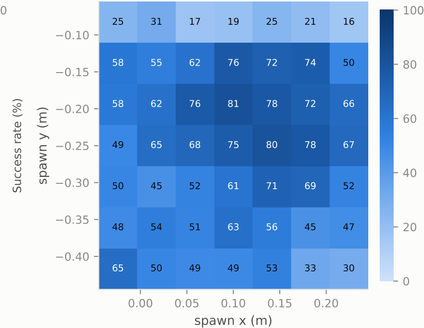
sac — success by spawn position
