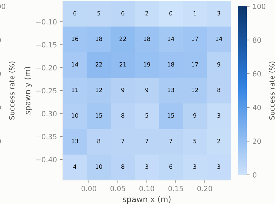
td3 — success by spawn position
