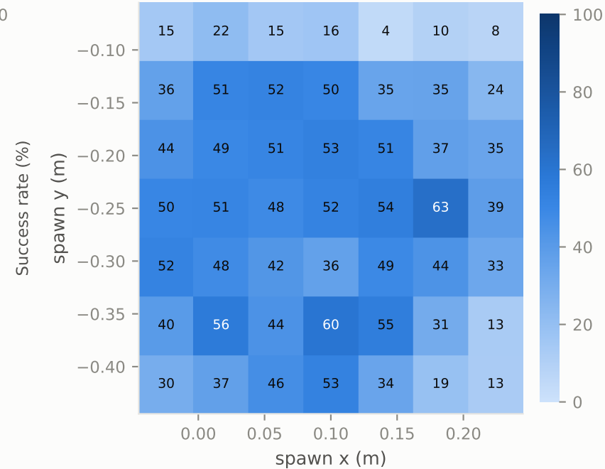
td3_In — success by spawn position
