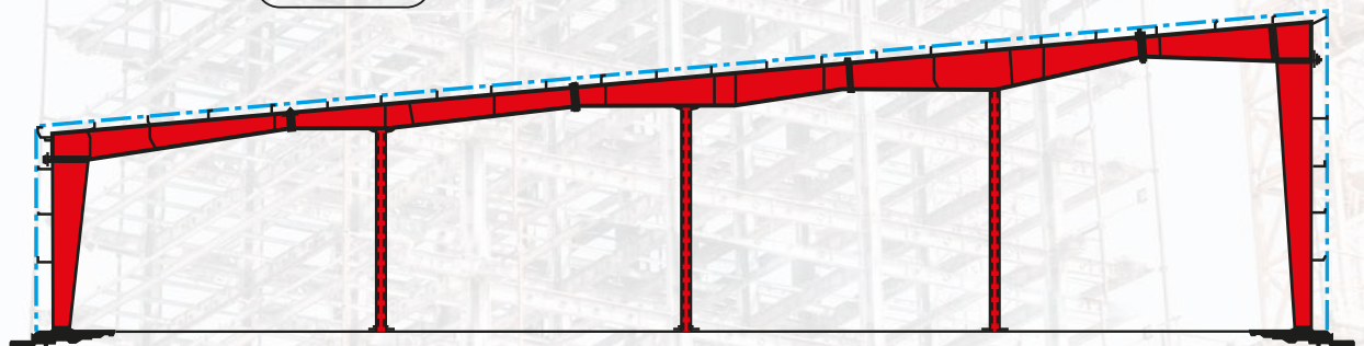
SECTION : MULTI-SPAN SINGLE SLOPE WITH FOUR SPANS
