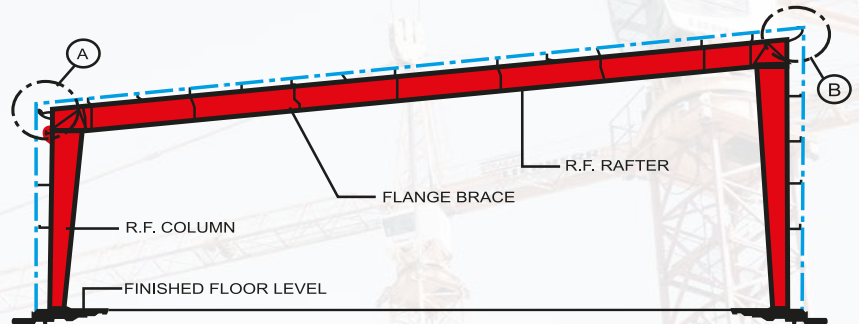
SECTION : SINGLE-SPAN SINGLE SLOPE
