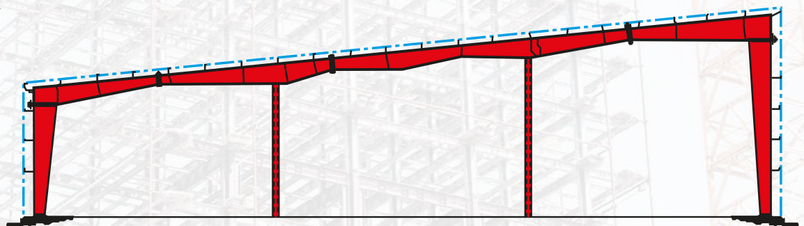
SECTION : MULTI-SPAN SINGLE SLOPE WITH THREE SPANS
