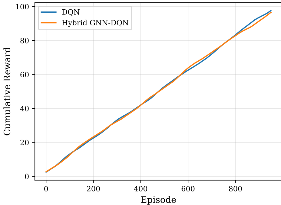
(b) RL Agent Reward
