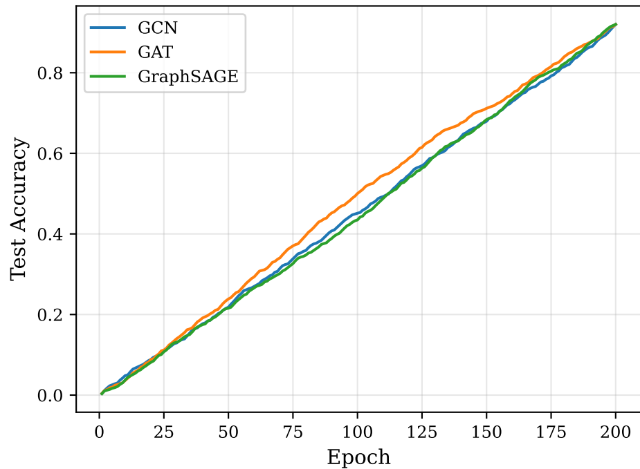
(a) GNN Model Accuracy
