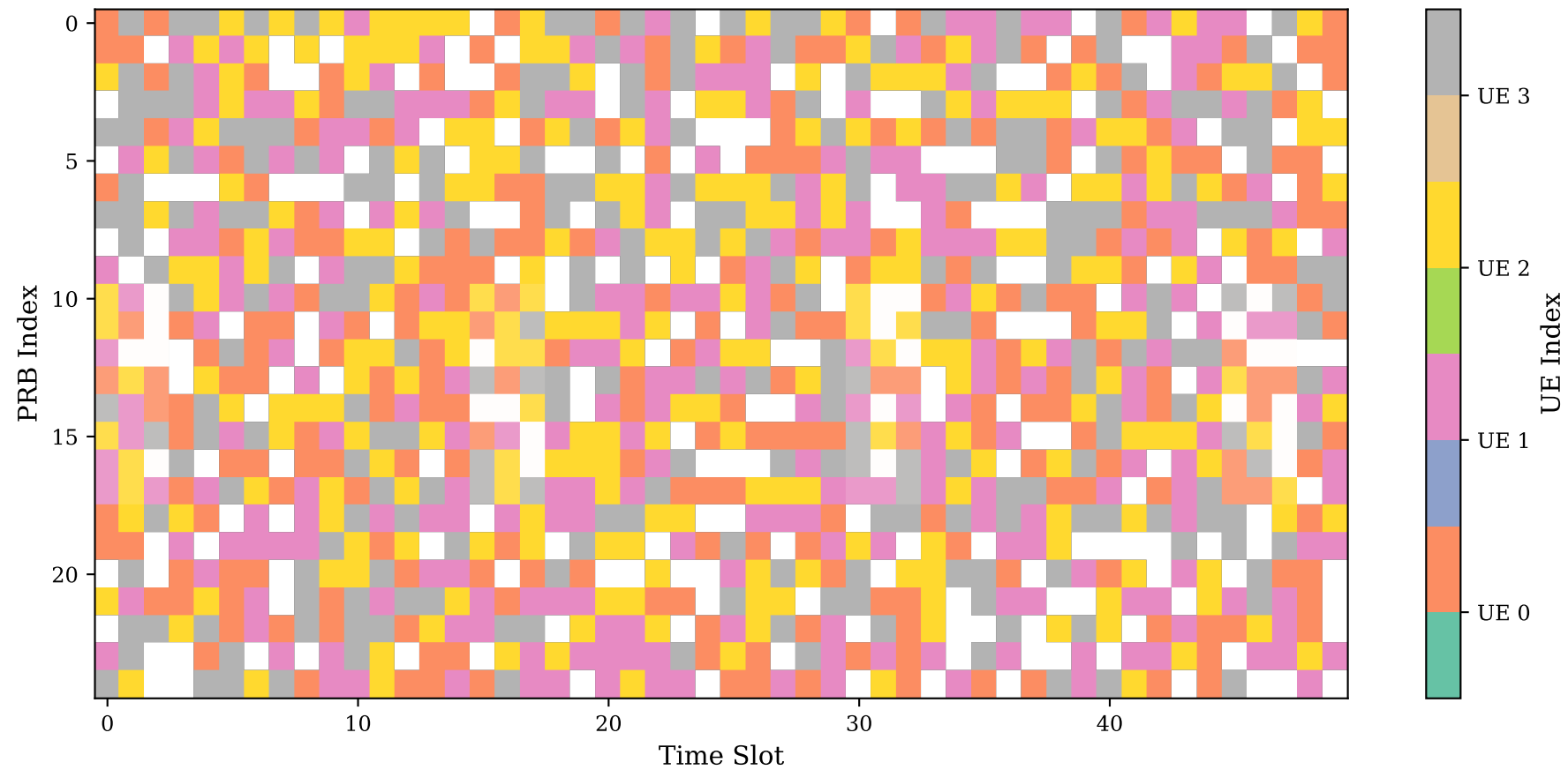
PRB Allocation Over Time
