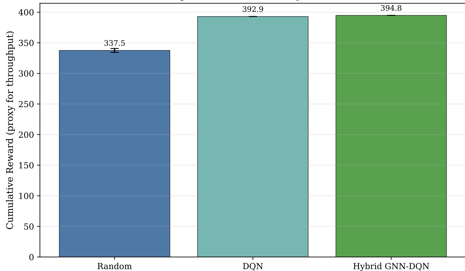
Agent Performance Comparison
