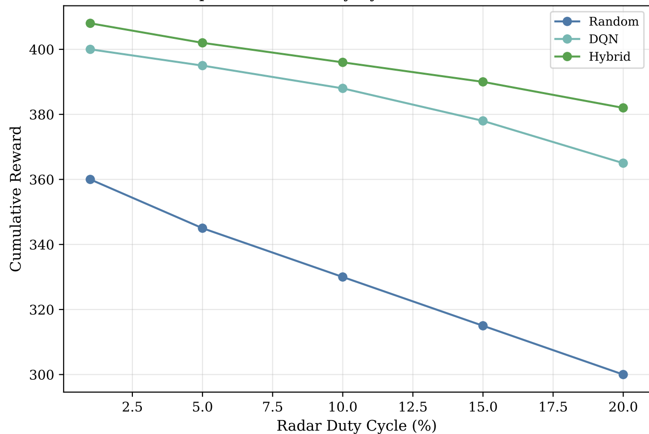
Impact of Radar Duty Cycle on Performance
