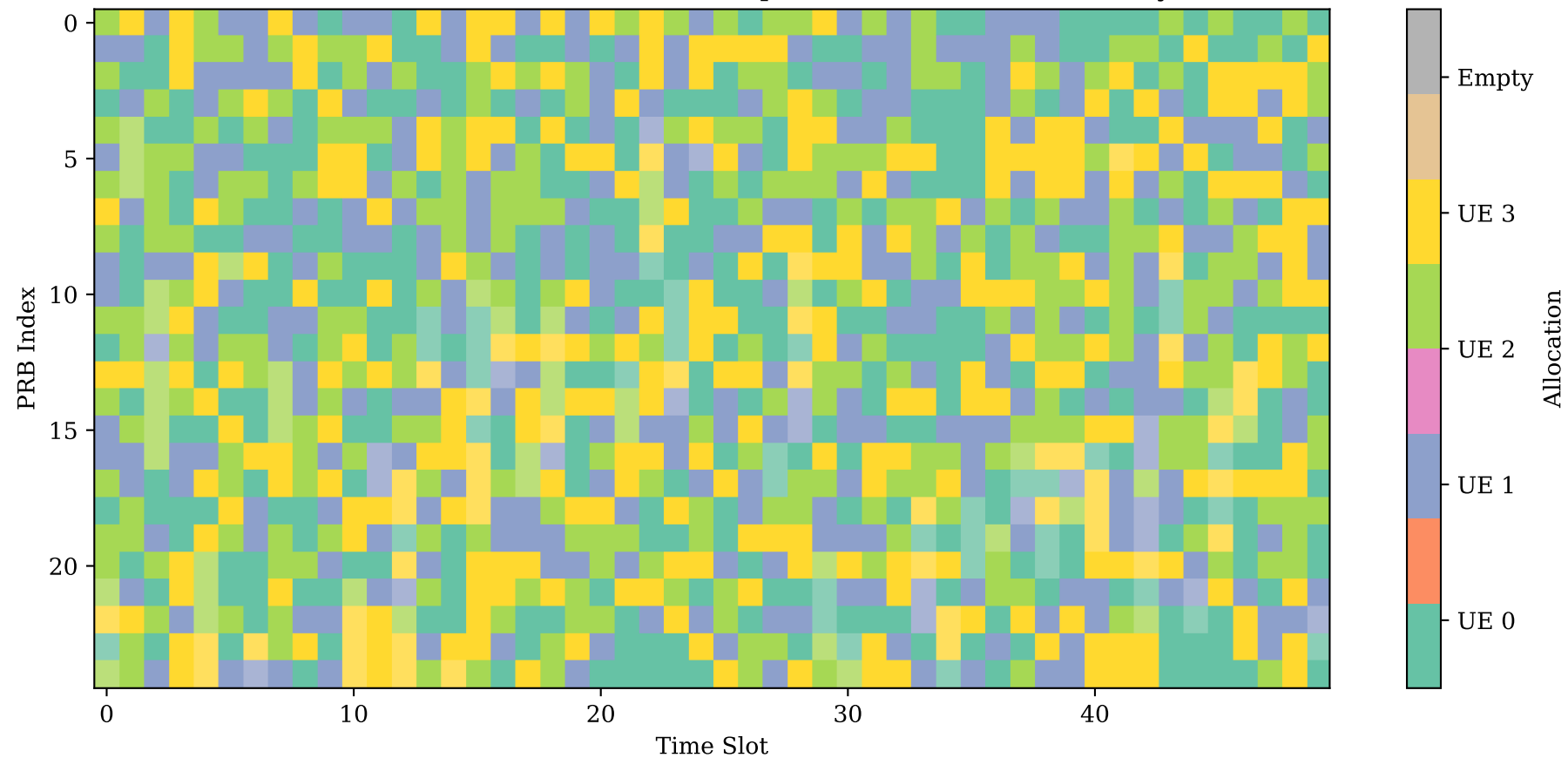
GNN-Predicted PRB Allocation (GraphSAGE) with Radar Overlay
