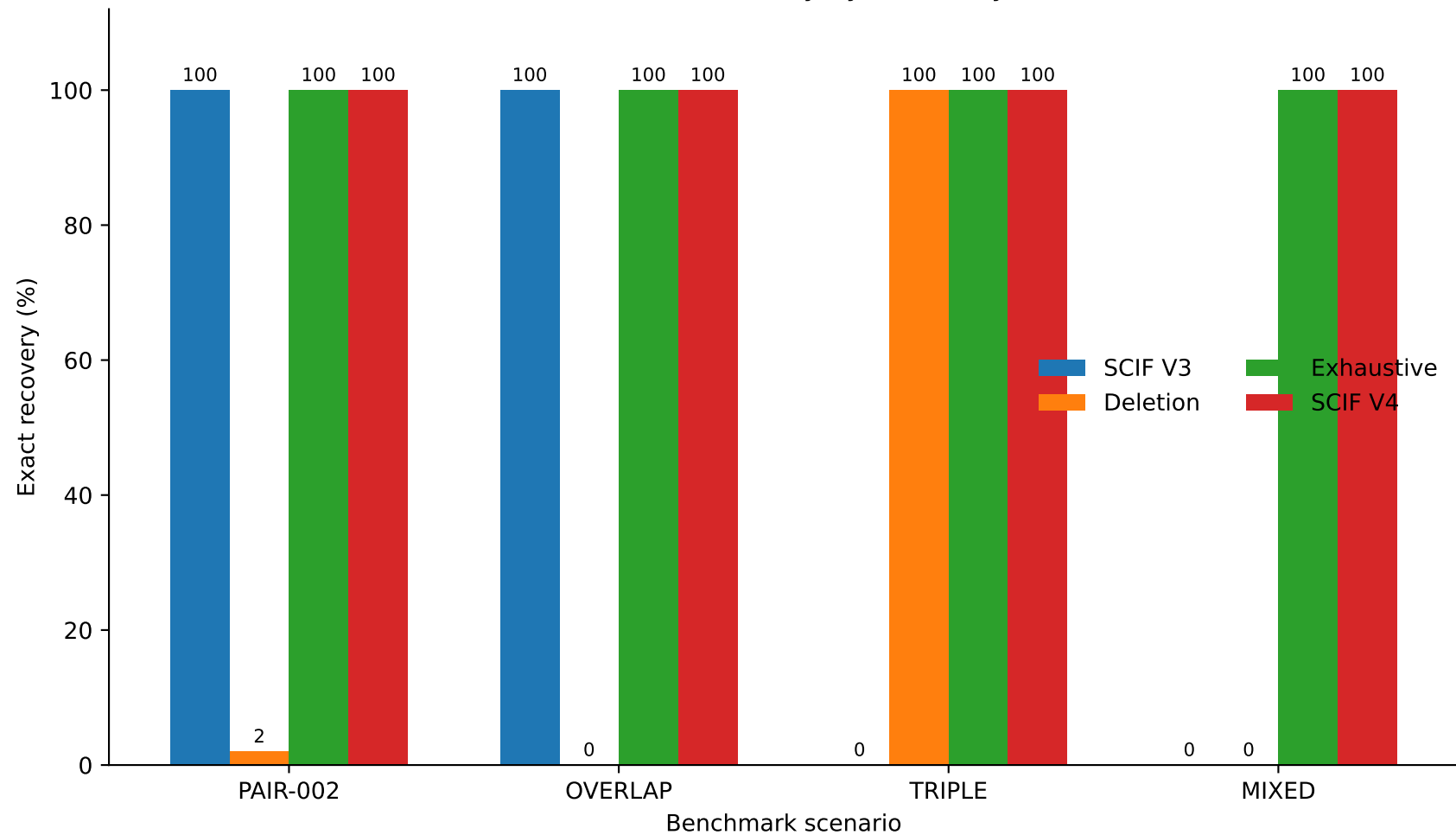
Exact Interaction Recovery by Discovery Method
