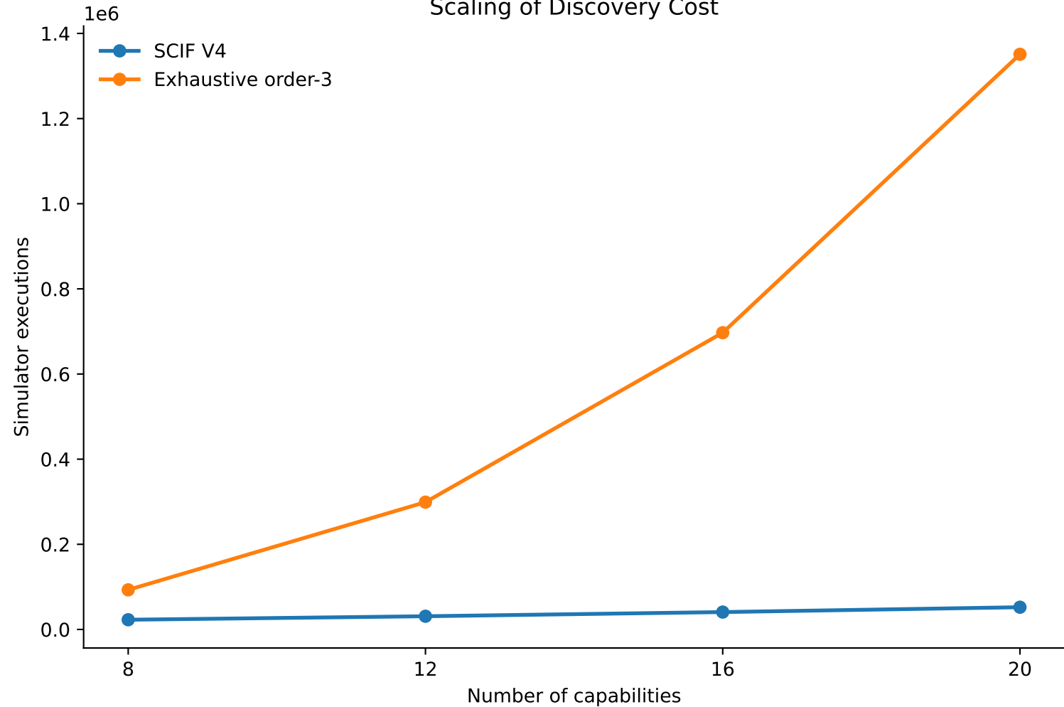
Scaling of Discovery Cost
