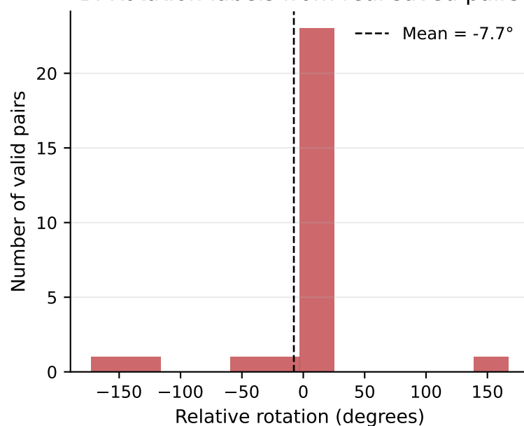
B. Rotation labels from real saved pairs
