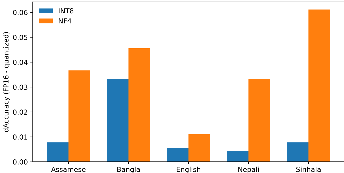
Quantization degradation by language - qwen2.5-3b-instruct
