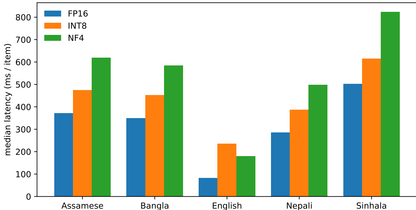
Latency - qwen2.5-3b-instruct (Tesla T4, within-session)
