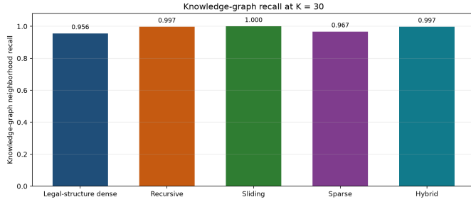
Fig. 3. Neighborhood recall legal graph pada K = 30 .
