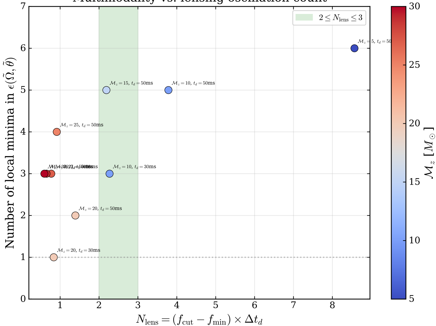
Multimodality vs. lensing oscillation count
