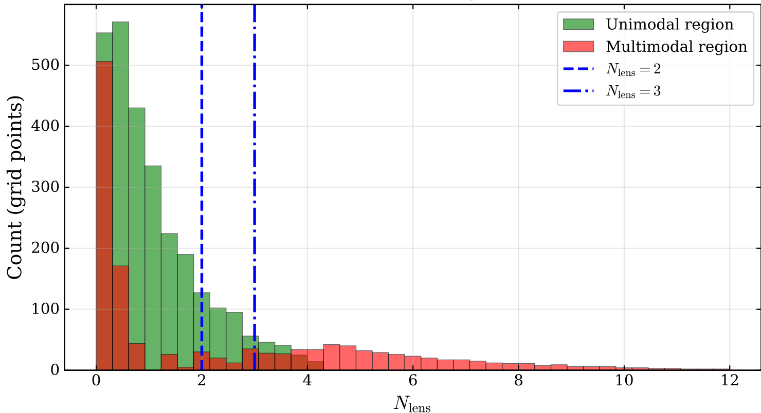
Distribution of N_{\text{lens}} by modality classification ( I = 0.5 , z = 1.0 , edge-on)
