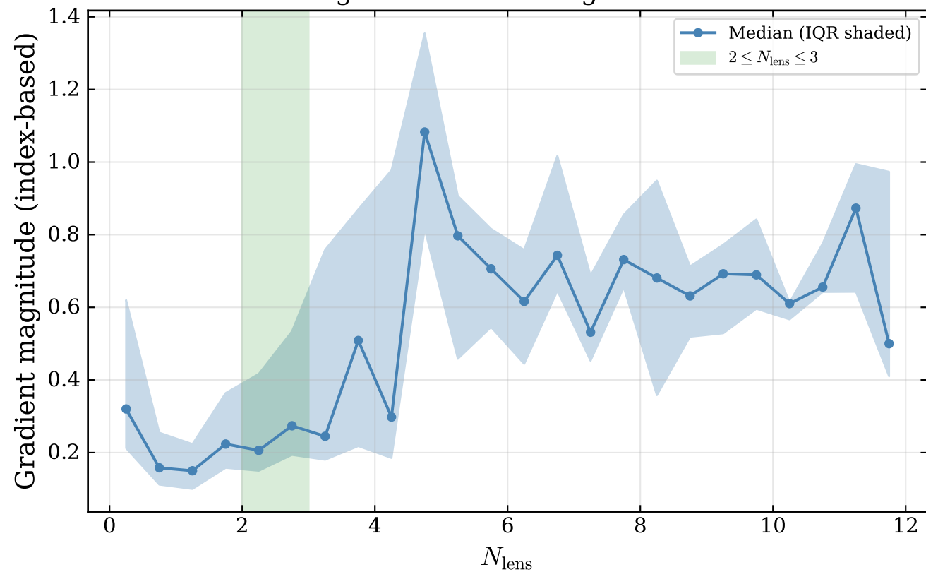
Parameter gradient vs lensing oscillation count
