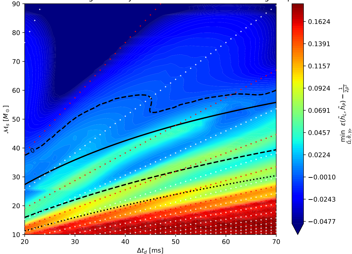
Lindblom Criterion: Distinguishability of Lensed Sources from Precessing Templates
