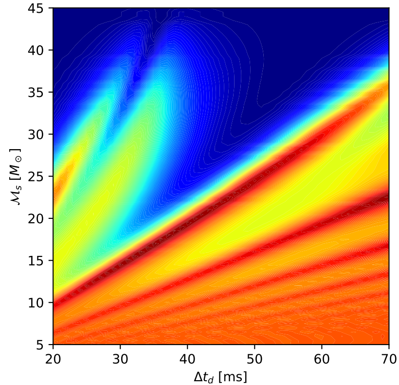
Lensed vs NP (super_contour, z=1)
