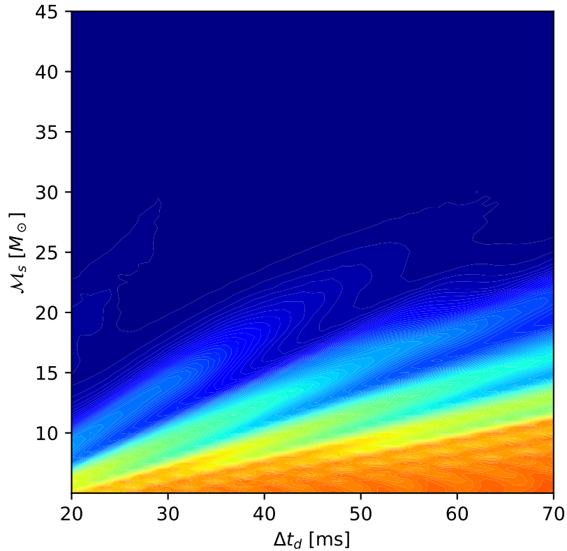
Lensed vs RP (best_match, z=1)
