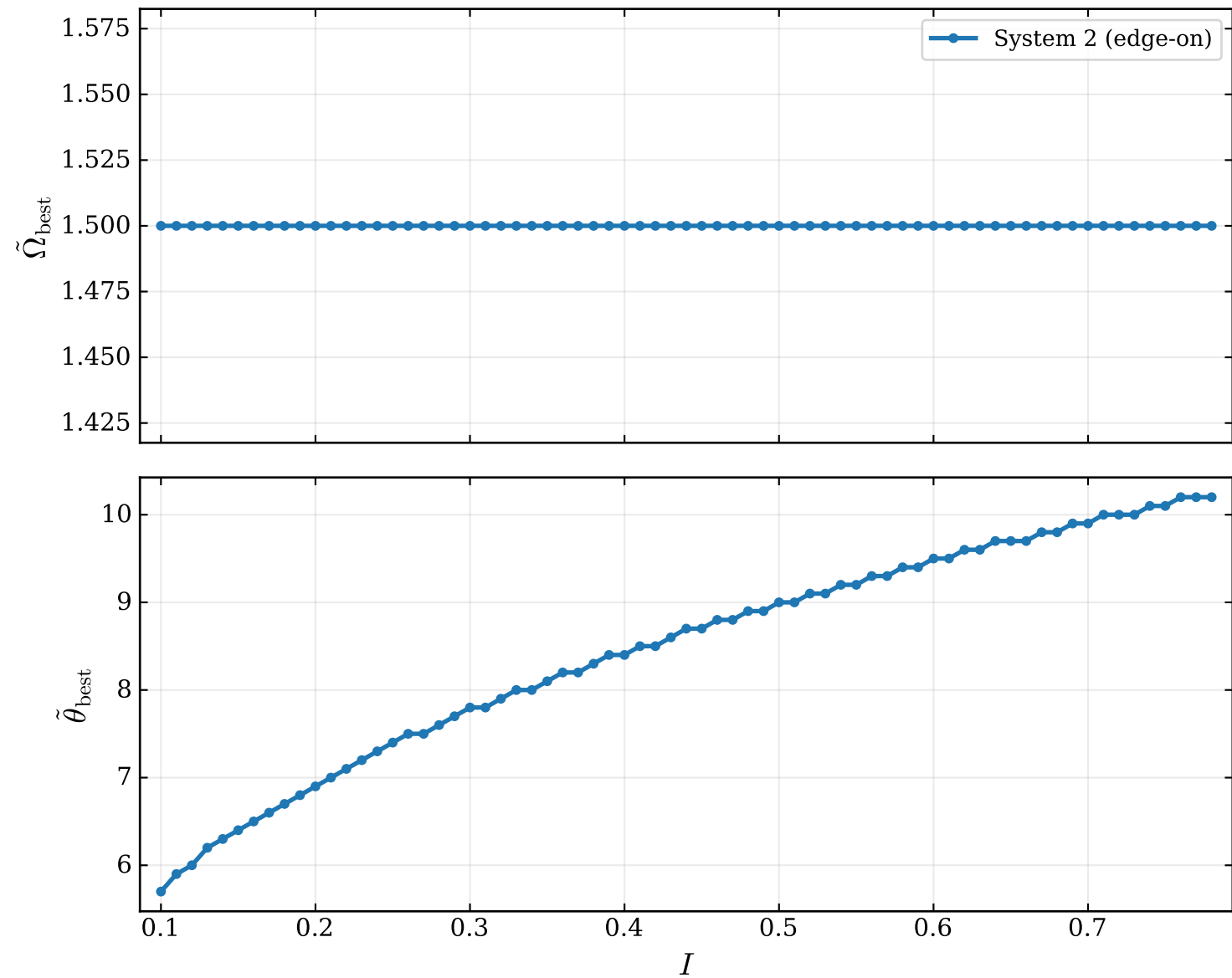
Best-matching precession parameters vs flux ratio ( \Delta t_{\text{d}} = 25 \text{ ms} , z = 1 , \mathcal{M}_{\text{s}} = 15 \text{ M}_{\odot} )
