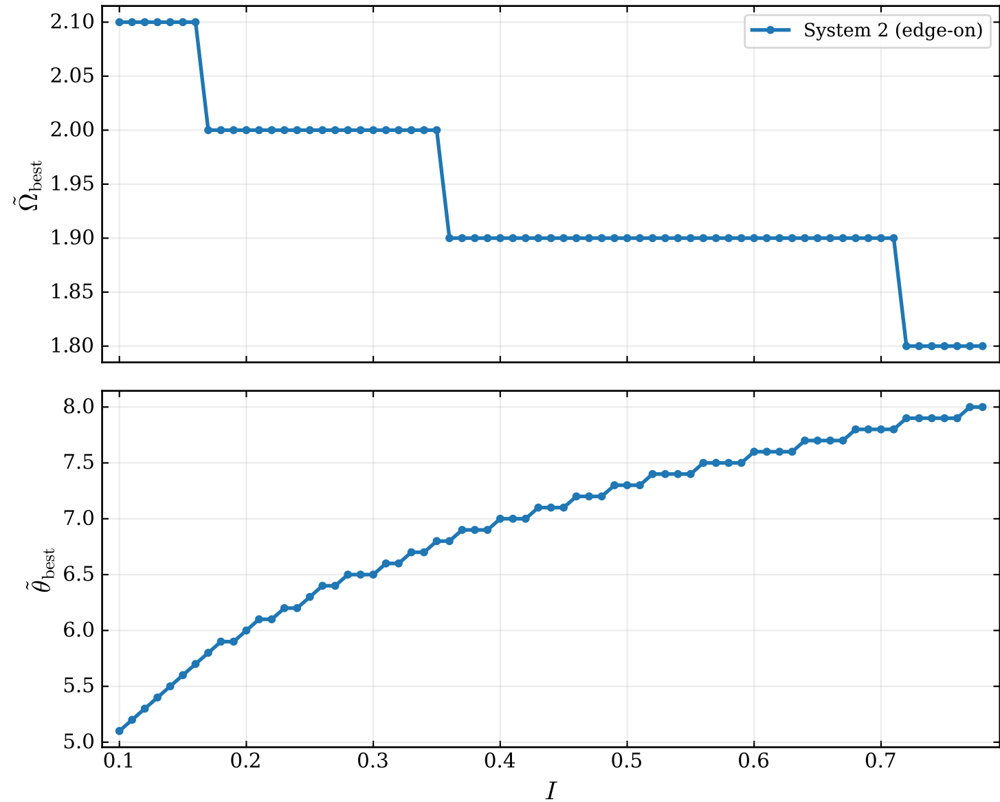
Best-matching precession parameters vs flux ratio ( \Delta t_d = 35 \text{ ms} , z = 1 , \mathcal{M}_s = 15 M_\odot )
