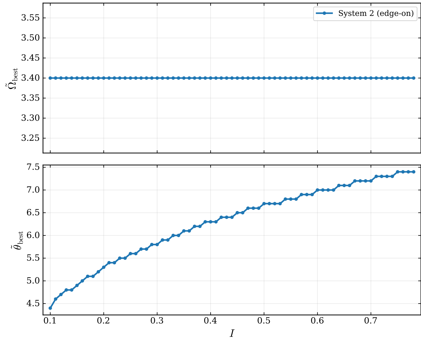
Best-matching precession parameters vs flux ratio ( \Delta t_d = 45 \text{ ms} , z = 1 , \mathcal{M}_s = 15 M_\odot )
