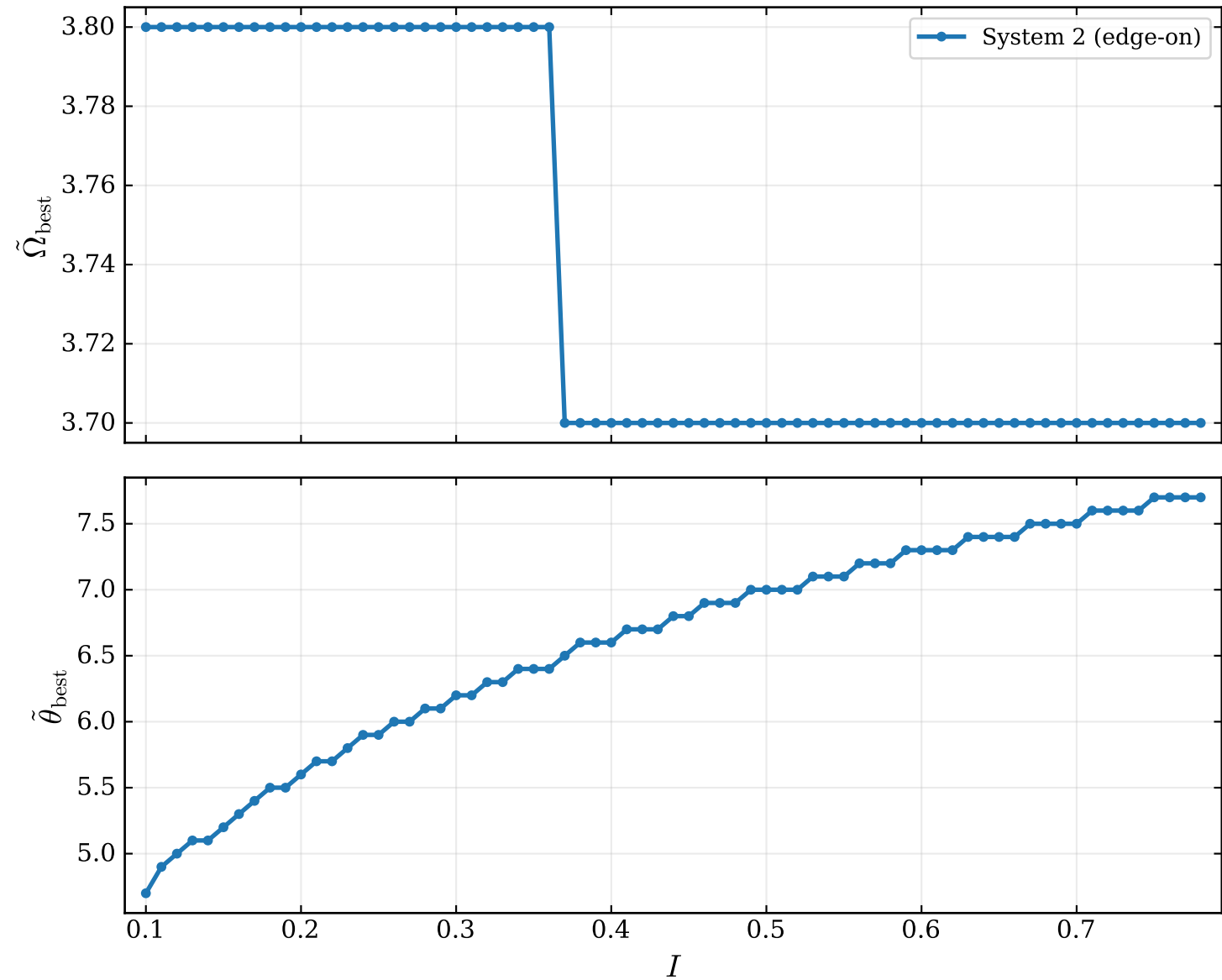
Best-matching precession parameters vs flux ratio ( \Delta t_d = 55 \text{ ms} , z = 1 , \mathcal{M}_s = 15 M_\odot )
