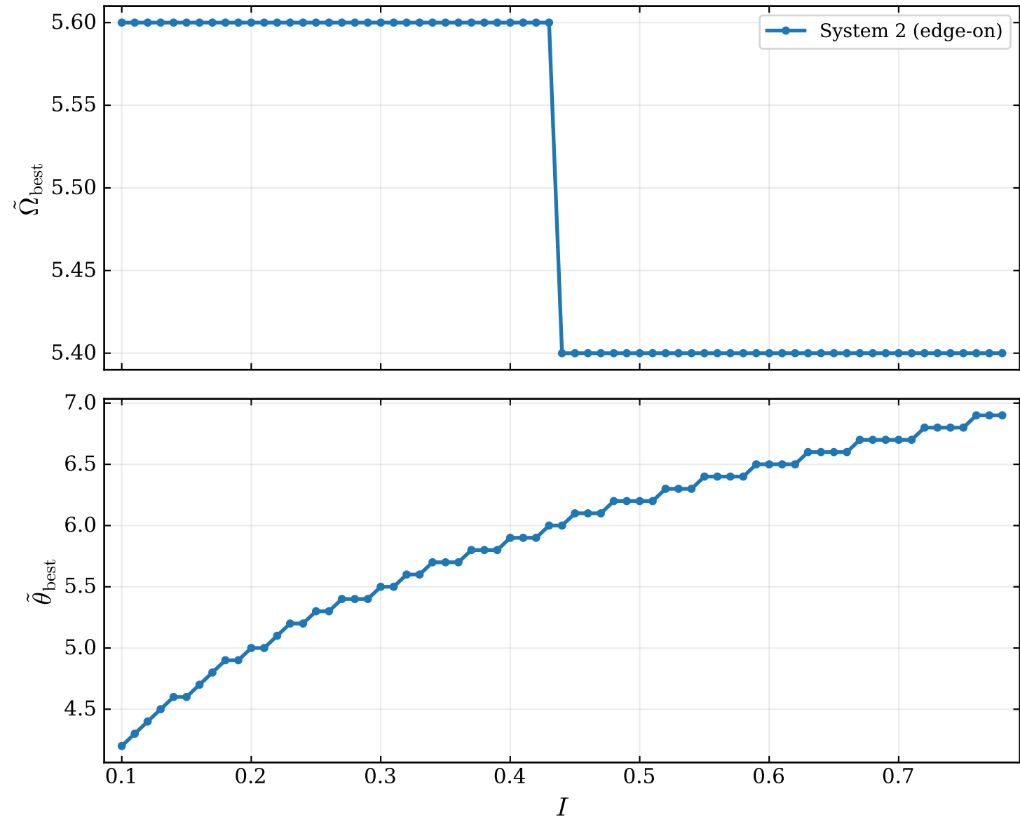
Best-matching precession parameters vs flux ratio ( \Delta t_d = 65 \text{ ms} , z = 1 , \mathcal{M}_s = 15 M_\odot )
