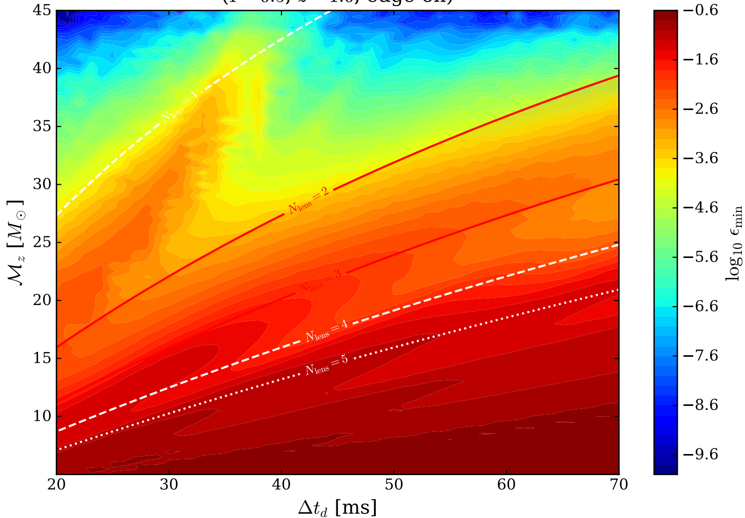
Minimum mismatch with N_{\text{lens}} contours ( I = 0.5 , z = 1.0 , edge-on)
