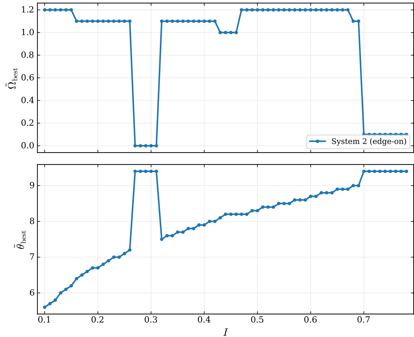
Best-matching precession parameters vs flux ratio (\Delta t_d = 20 \text{ ms}, z = 1, \mathcal{M}_s = 15 M_\odot)
