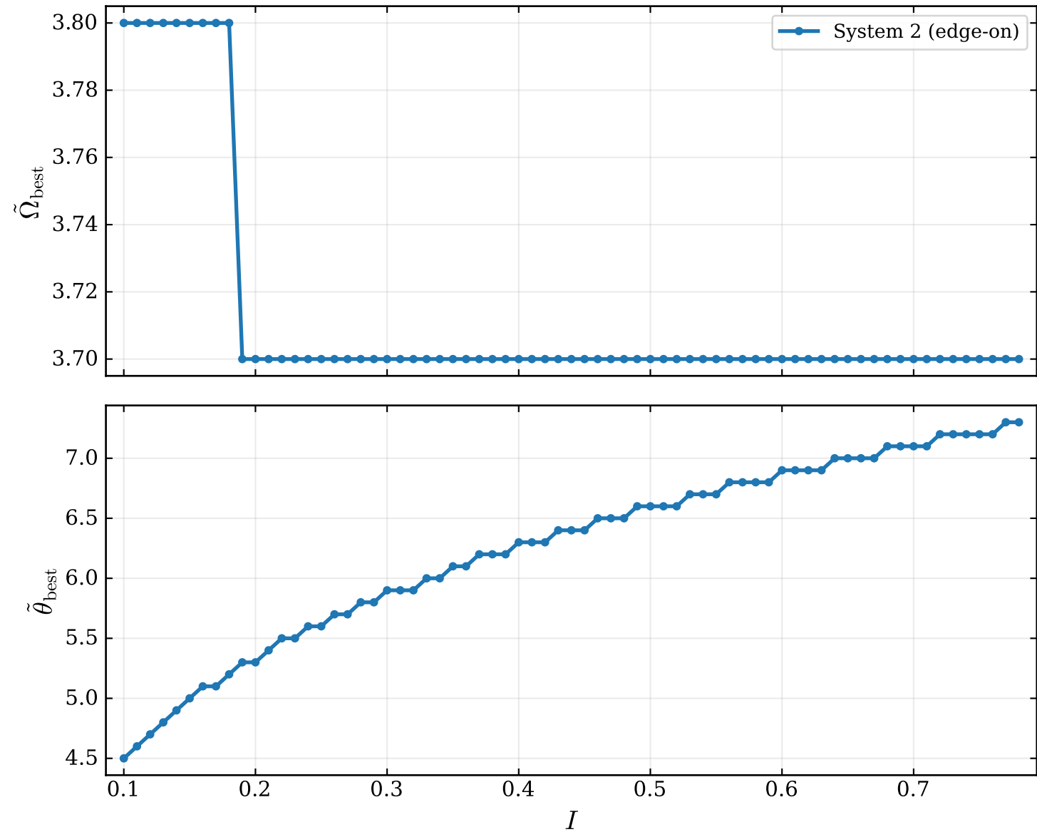
Best-matching precession parameters vs flux ratio ( \Delta t_{\text{d}} = 50 \text{ ms} , z = 1 , \mathcal{M}_{\text{s}} = 15 M_{\odot} )
