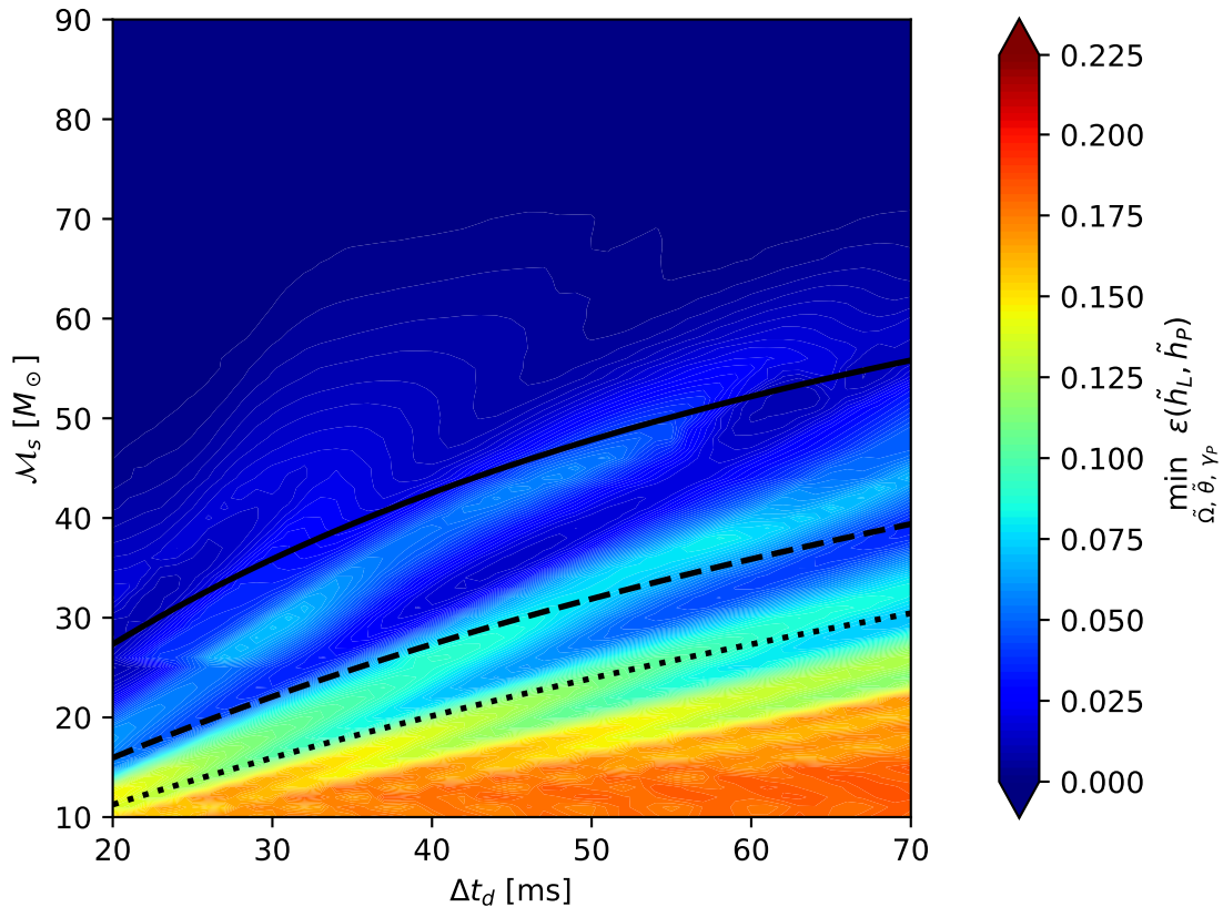
Lensed Sources vs Regularly Precessing Templates
