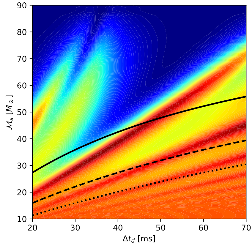
Lensed Sources vs Non-Precessing Templates
