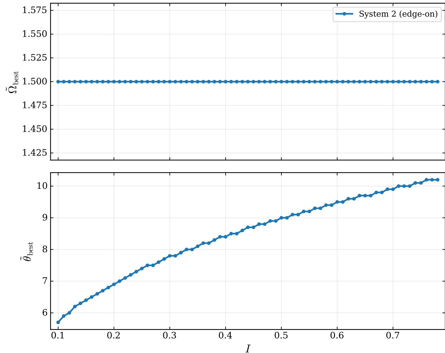
Best-matching precession parameters vs flux ratio ( \Delta t_{\text{d}} \approx 25 \text{ ms} , z = 1 , \mathcal{M}_{\text{s}} = 15 \text{ M}_{\odot} )
