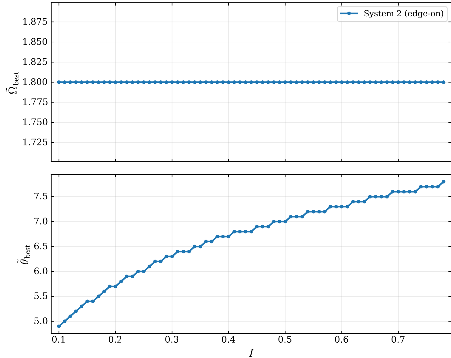
Best-matching precession parameters vs flux ratio ( \Delta t_{\text{d}} \approx 30 \text{ ms} , z = 1 , \mathcal{M}_{\text{s}} = 15 \text{ M}_{\odot} )
