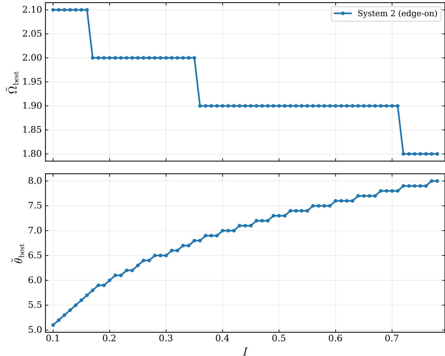
Best-matching precession parameters vs flux ratio ( \Delta t_d \approx 35 ms, z = 1 , \mathcal{M}_s = 15 M_\odot )
