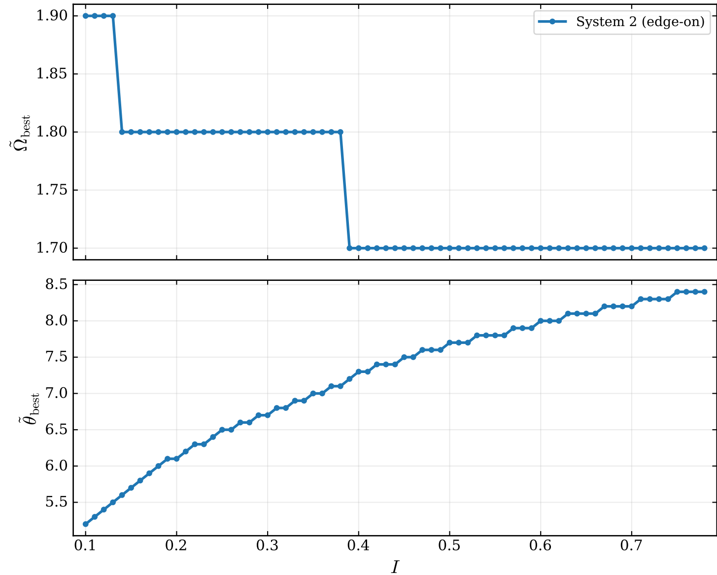
Best-matching precession parameters vs flux ratio ( \Delta t_d \approx 40 \text{ ms} , z = 1 , \mathcal{M}_s = 15 M_\odot )
