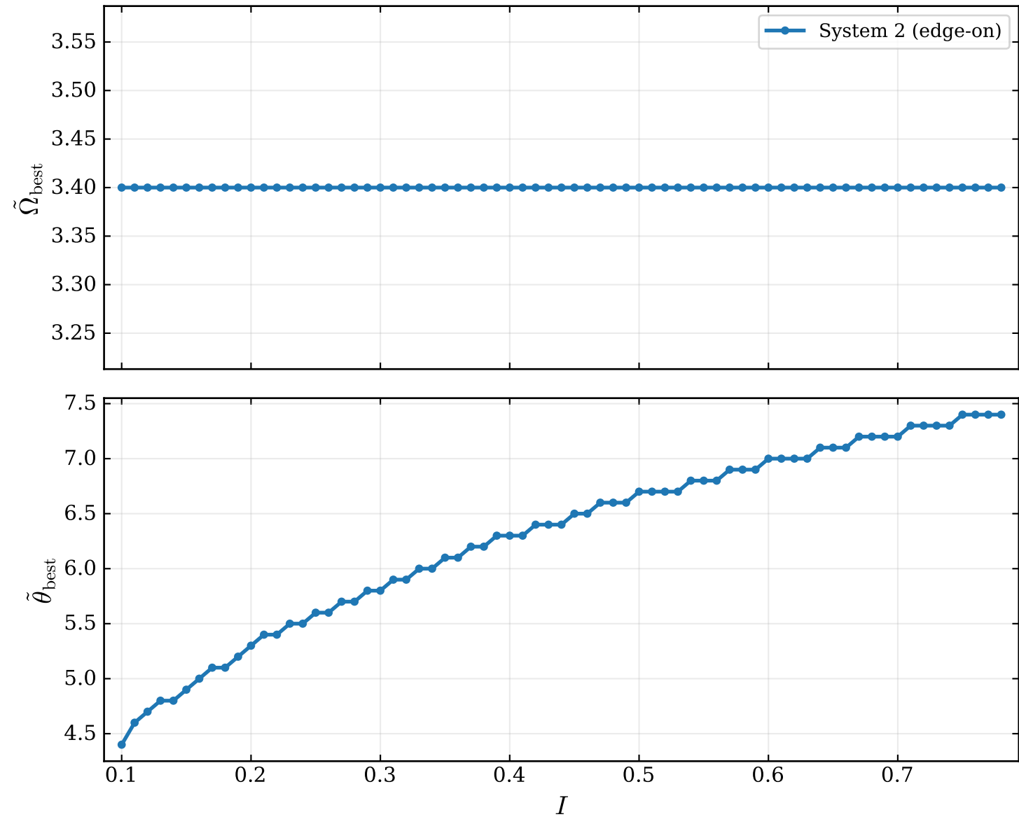
Best-matching precession parameters vs flux ratio ( \Delta t_{\text{d}} \approx 45 \text{ ms} , z = 1 , \mathcal{M}_{\text{s}} = 15 M_{\odot} )
